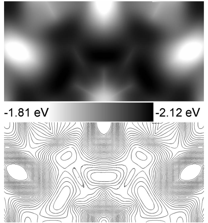
FIG. 7. Potential map of one CuPc on a C 60 layer. The scanned area is 1.0 \times 0.5 nm 2 . As the contrast of the grayscale plot is not that good in the energetically favorable regions, a contour plot is given below.
