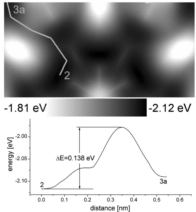
FIG. 11. Potential map of one CuPc on a C_{60} layer. A path leading from an energetically favorable position to a local minimum belonging to the neighboring C_{60} molecule is marked; the potential energy along this path is plotted below.
