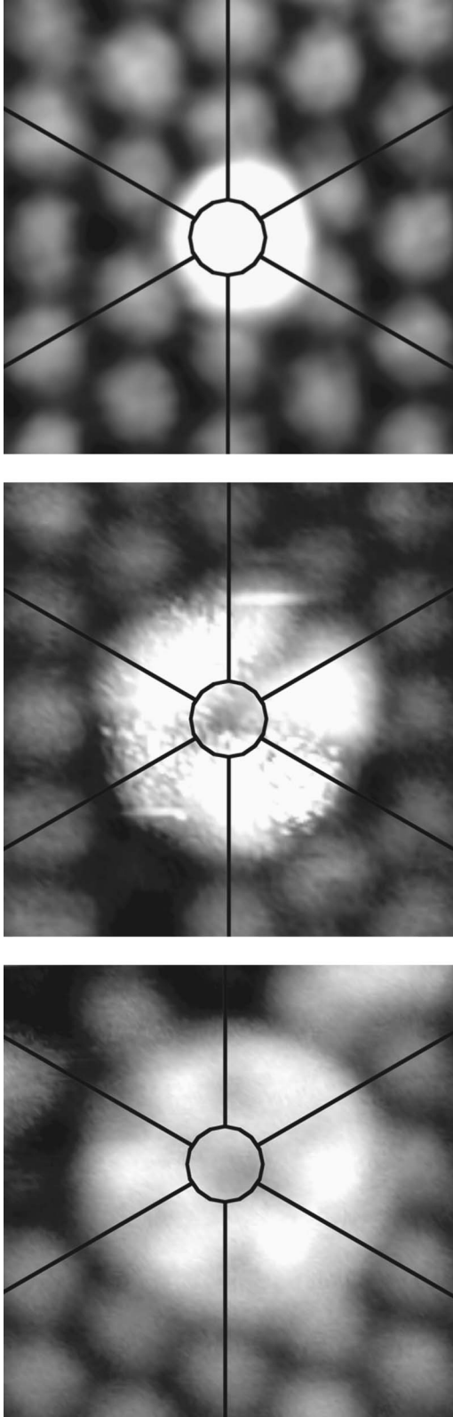
FIG. 3. STM images of a single CuPc molecule on top of a C 60 layer at different temperatures. The displayed areas are 5 \times 5 \text{ nm}^2 . All images were corrected for thermal drift. The black drawings within the images indicate the central C 60 molecule and the directions of the unit cell vectors. For the image taken at 50 K, the CuPc is not adsorbed symmetrically on top of the underlying C 60 molecule.
