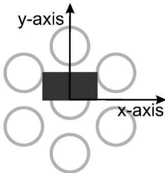
FIG. 6. Sketch of the scanned area: The circles mark the positions of the C 60 molecules, the rectangle indicates the scanned area of 1.0 \times 0.5 nm 2 . For the calculations, Cartesian coordinates with the axes given in the sketch are used.
