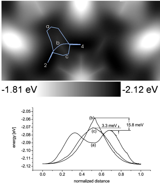
FIG. 9. In addition to the favorable path (a) (see Fig. 8), two other reasonable paths are marked, a circle line (b) and a path that is obtained when we start the NEB algorithm with different initial intermediate points (c). The potential energy along the three paths is plotted below, the path length has been normalized. One can see that path (c) has a slightly higher potential energy than path (a). The increase is less than 8%.
